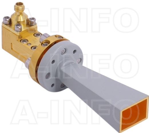
LB-15-15-C-1.0F Standard Gain Horn Antenna 50-75GHz 15dB Gain 1.0mm Female
